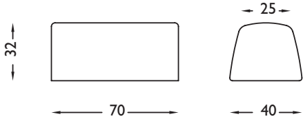
COUNTERWEIGHTED BACKREST
